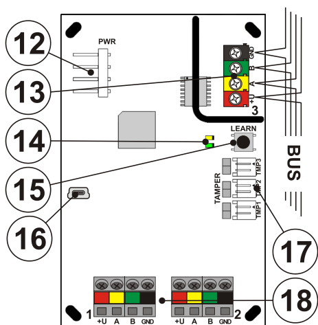
Figure 4: 12 – power terminal from power supply; 13 – BUS input terminals; 14 – LED indicators; 15 – LEARN (enroll) button; 16 – USB connector; 17 – connectors for tamper contacts; 18 – BUS output terminals
