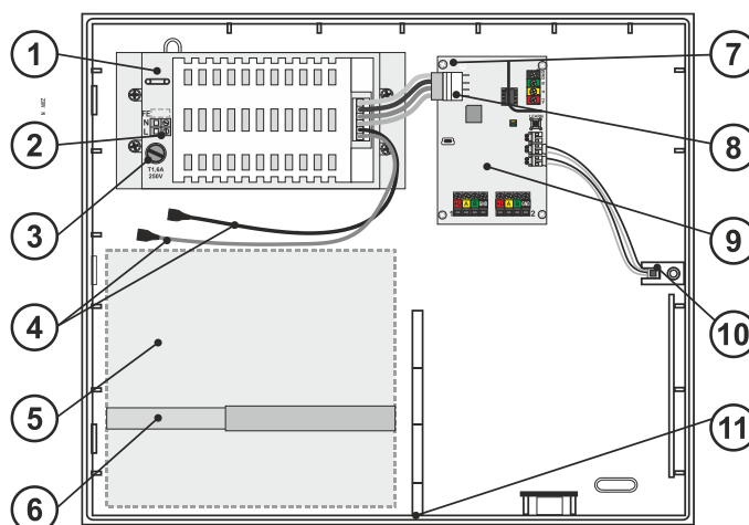
Figure 3: 1 – mains power supply; 2 – mains power terminals; 3 – mains power fuse (T1.6 A); 4 – back-up battery connecting cables; 5 – back-up battery; 6 – belt clip to fix the back-up battery; 7 – screws to fix the PCB into the installation box; 8 – connecting terminal from power supply; 9 – the JA-120Z PCB; 10 – front and rear tamper contact of the box; 11 – PLV-CP-L plastic housing
