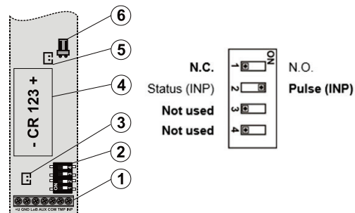
Fig. 2 – Transmitter JA-150TX-VX1: 1 – wire terminals, 2 – settings DIP switch (pre-set from factory, see picture), 3 – external tamper contact jumper, 4 – battery holder, 5 – external antenna jumper, 6 – external antenna connector
