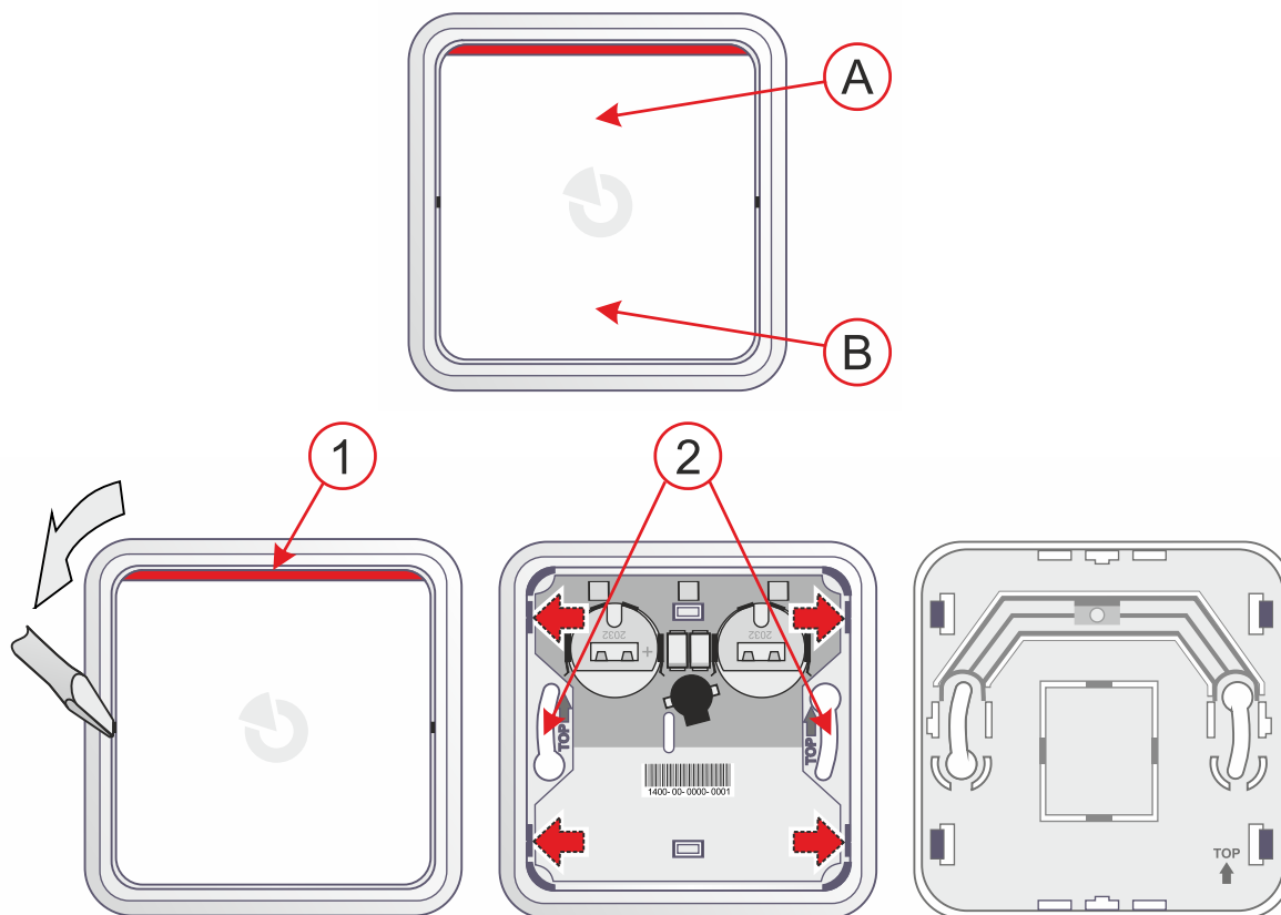
Fig. 1: Description of external parts of the product and layout of the button into 3 parts A, B – buttons; 1 – LED; 2 – holes for fixing screws;
