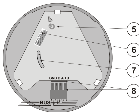
Figure 2: 5 – alignment arrow / logo; 6 – production number; 7 – tamper sensor; 8 – BUS connection terminal
