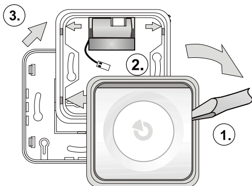
Figure 1: Disassembly of the siren before installation
